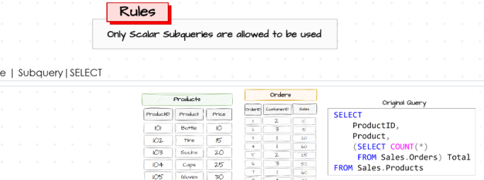
SQL Course | Subquery | SELECT
