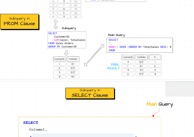
SQL Course | Subquery | FROM
