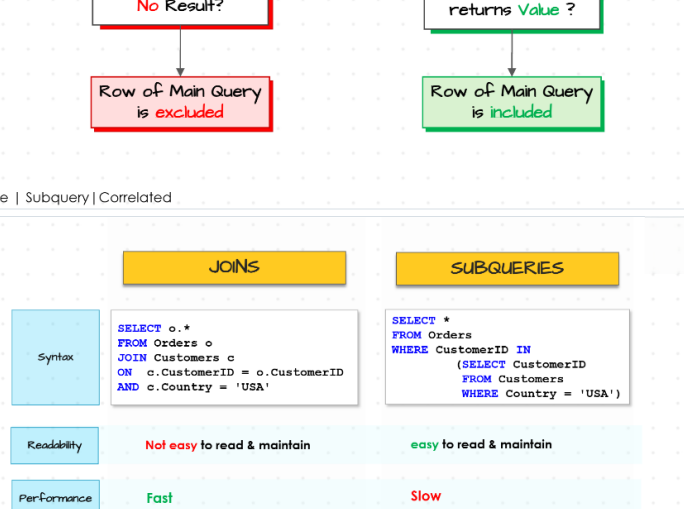
SQL Course | Subquery | Correlated
